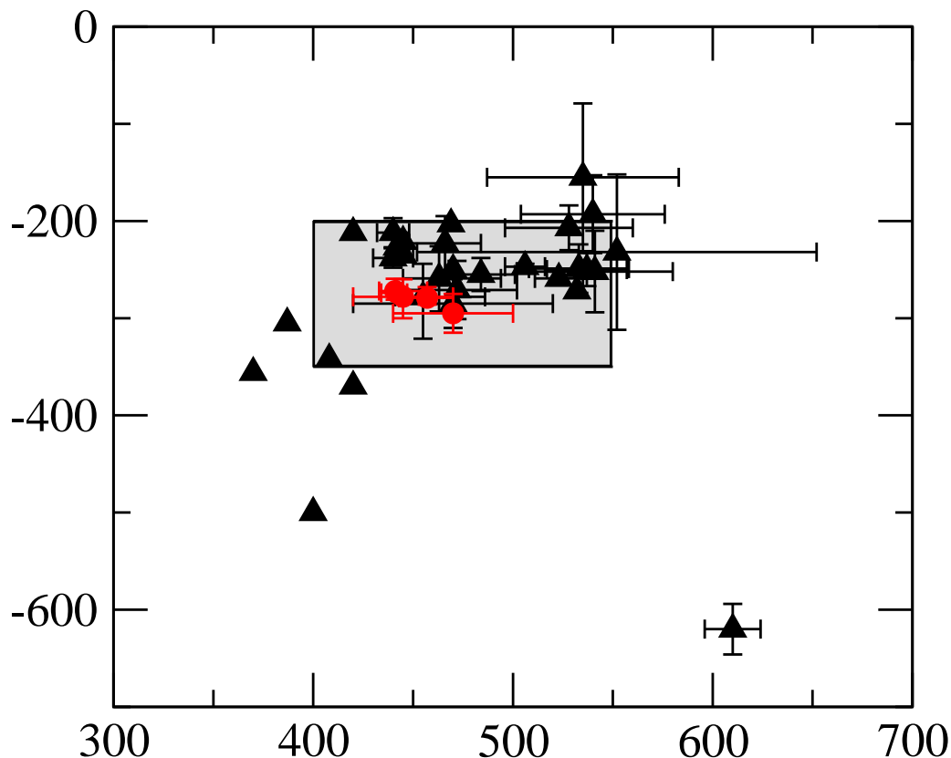
Figure 74.1: Location of the f_0(500) (or \sigma ) poles in the complex energy plane. Circles denote the recent analyses based on Roy(-like) dispersion relations [9–12], while all other analyses are denoted by triangles. The corresponding references are given in the listing.
